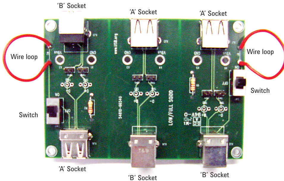
Figure 2. Keysight SQuIDD board.
