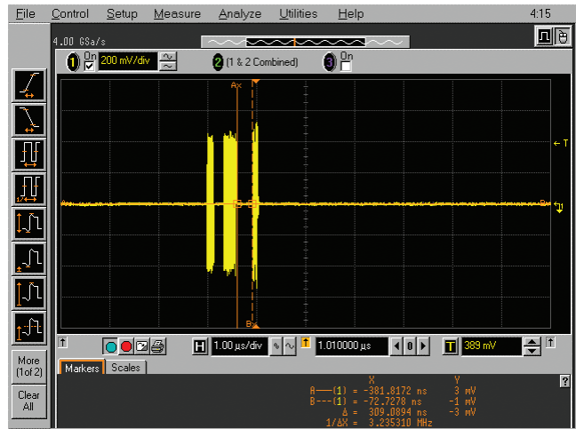
Figure 13. Device inter-packet gap.
