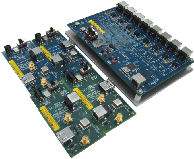
Figure 10. Hi-speed signal quality boards (Keysight fixture and Intel fixture—device signal quality test).
